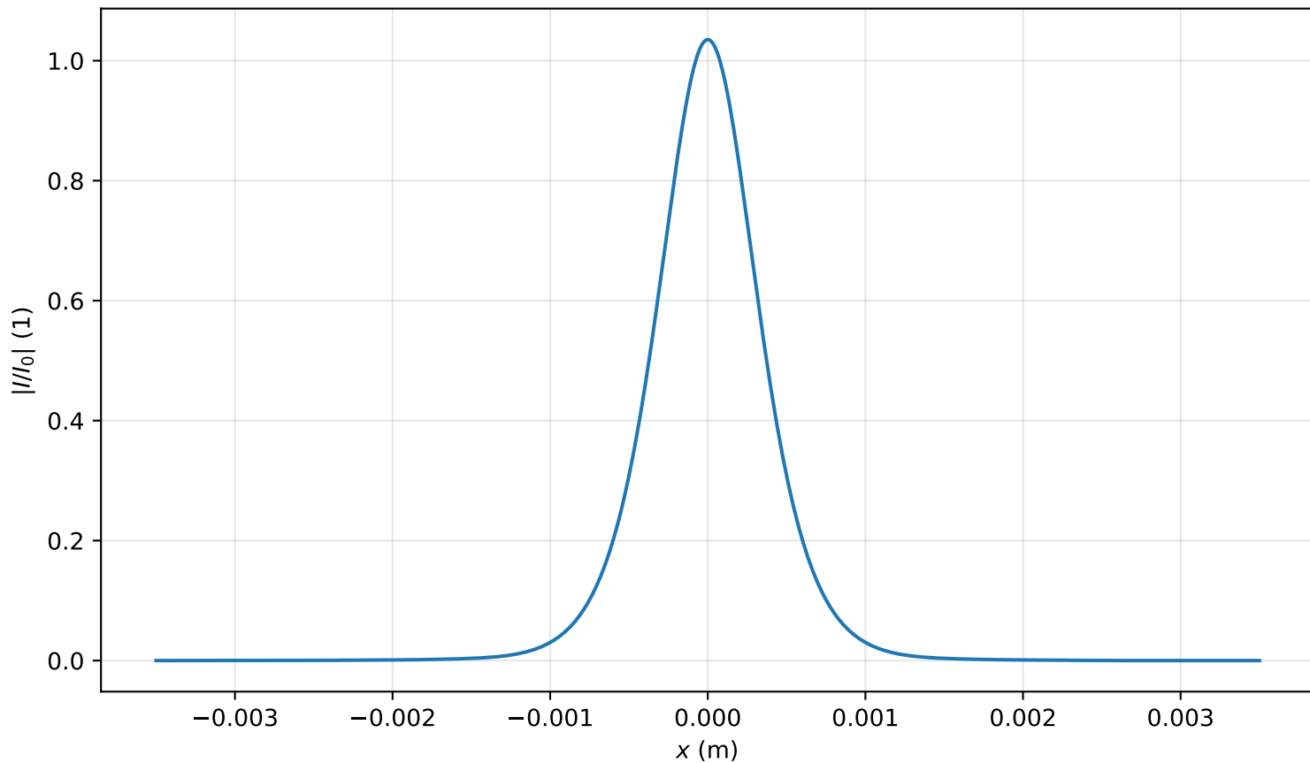
Intensity profile I(x, y = 0, z = 3.264m)/I_0 , P_{in}=0.8P_{cr} , artificial time
